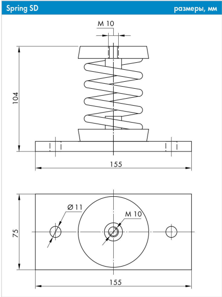
Vibrofix Spring SD
